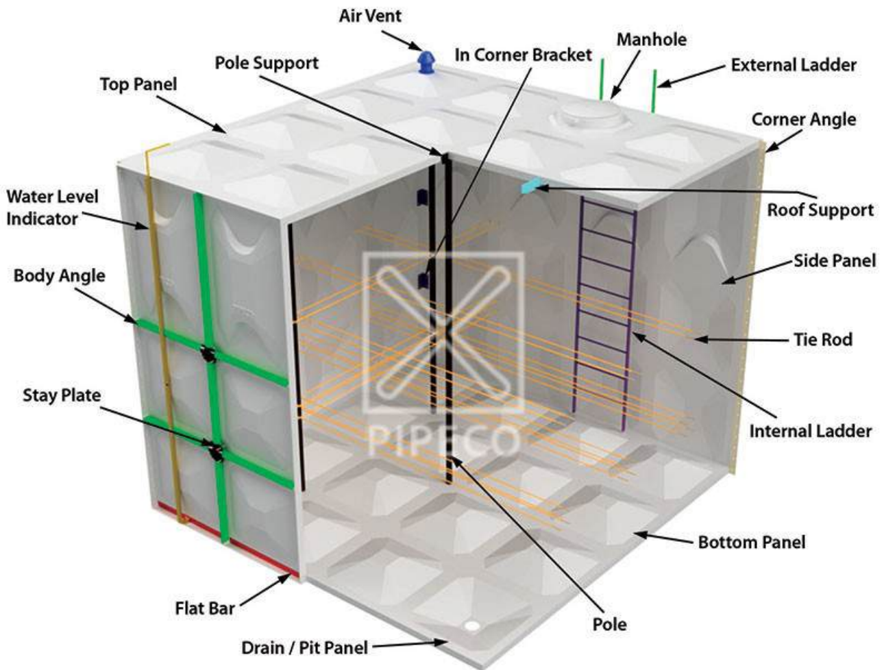
*4m x 4m x 3.5m(H) GRP sectional water tank illustration
